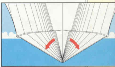
One way to look at how the SeaV 2 hull works is to envision a series of wedges. The flatter aft sections create lift, stability, and efficiency as the boat drives through the water.
