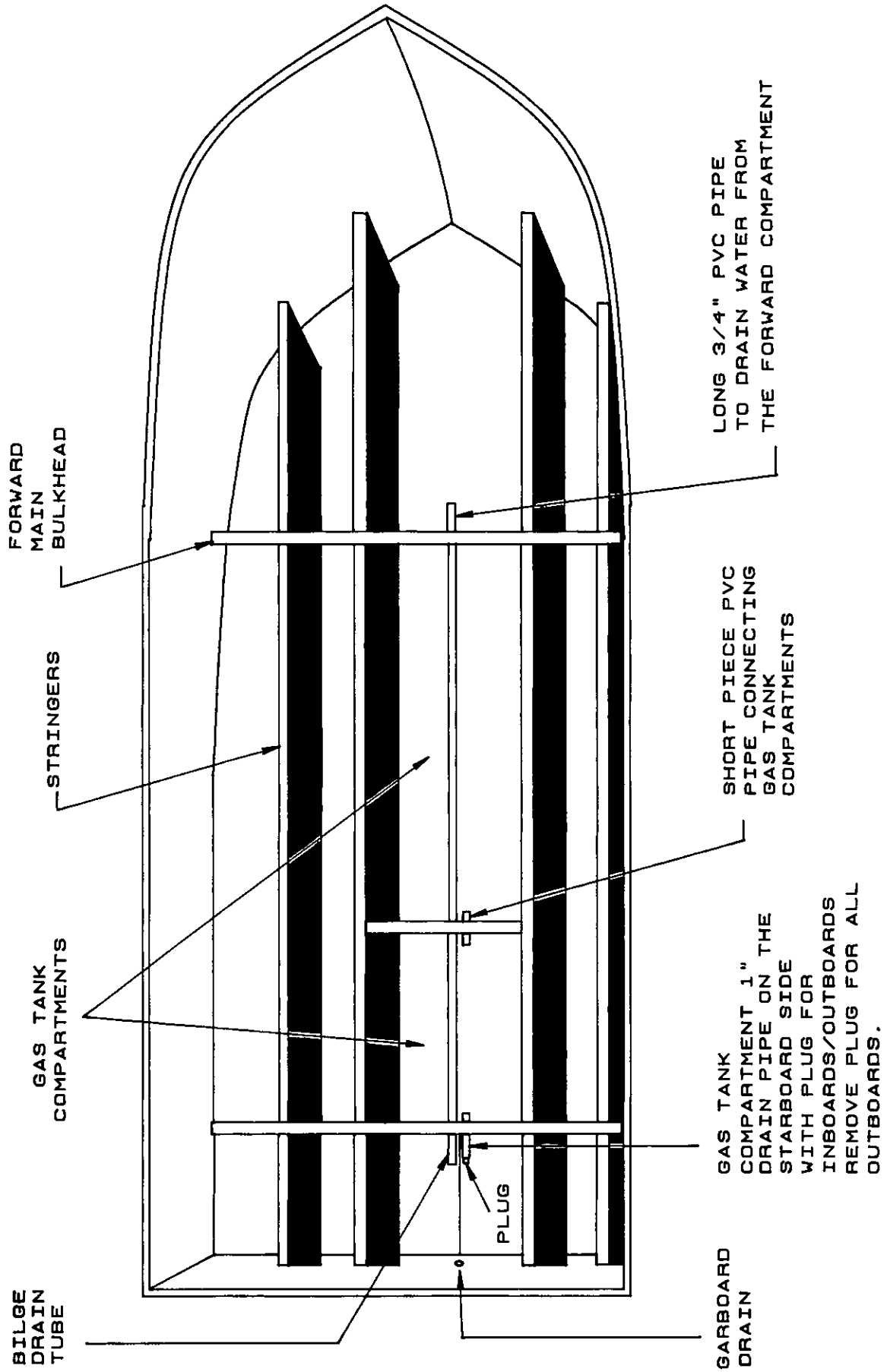
TYPICAL FUEL TANK DRAINAGE
